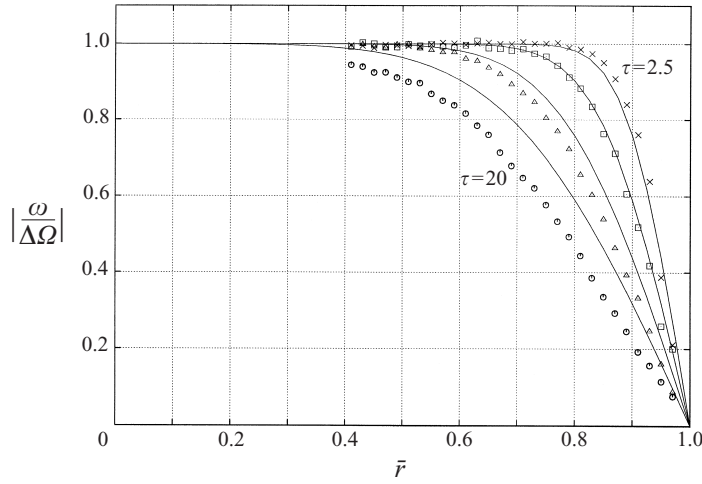
FIGURE 13. A comparison between experiment and boundary-layer analysis predictions at \tau = 2.5, 5, 10, 20 . \Delta\Omega = |\Omega_i - \Omega_f| , \Omega_i = \pi/4 \text{ s}^{-1} , \Omega_f = \pi/5 \text{ s}^{-1} (spin-down) N^2 = 4.4 \text{ s}^{-2} ( \hat{W}_e = 5/4 , S^* = 11.2 + \hat{W}_e^2 ). Numerical results are obtained with \sigma = 700 .
